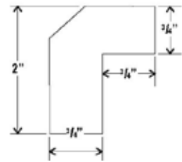
Angle Light Rail Moulding ALRM8
