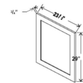
Base Decorative Door Panel BDEP
