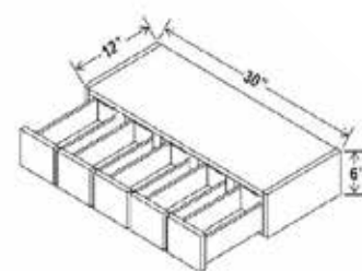
Wall Spice Drawer WSD3630 5 drawers
