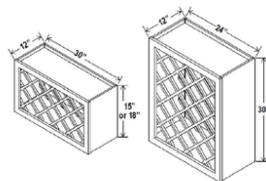
Wine Rack WRC2430 WRC3015 WRC3018 Can install vertically or horizontally
