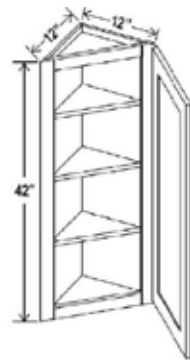
Angle Wall Cabinet AW1242
