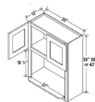
Microwave Wall Cabinet MO3030 MO3036 MO3042
