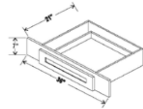
Knee Drawer VKD36
