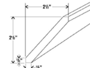
Angle Crown Moulding
