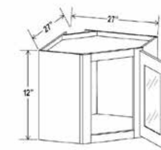
Diagonal Corner Wall Cabinet Glass Door
