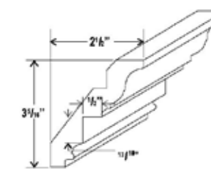
Insert Crown Moulding
