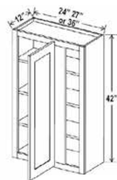
Wall Blind Corner Cabinet 42" H WBC2442 WBC2742 WBC3641 Can be pulled to exact fit
