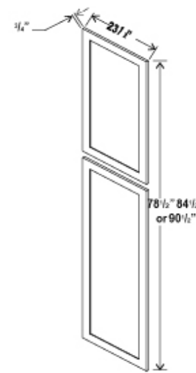
Tall Decorative Door Panel TDEP2484 TDEP2490 TDEP2496
