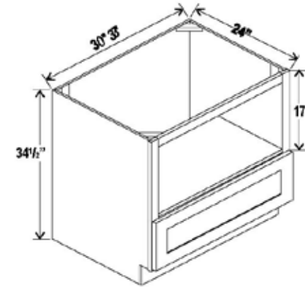
Microwave Base Cabinet MB30 MB33
