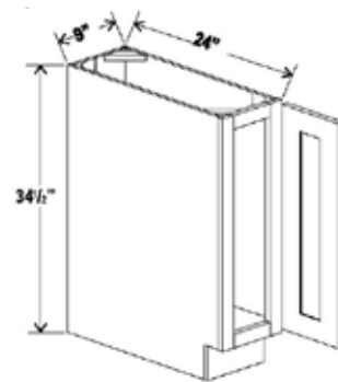
Base Tray BT09
