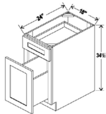
Base Waste Basket Cabinet BWB18
