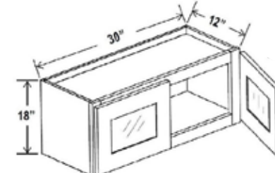
Wall Cabinet Double Glass Doors 18" H
