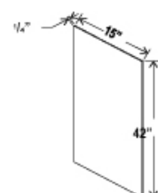
Wall Skin Panel WSV42
