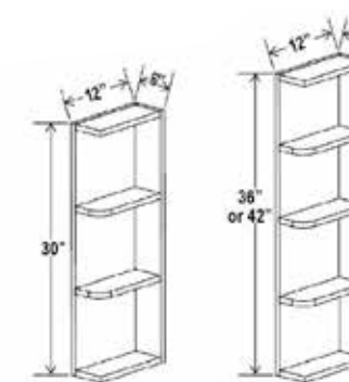
Open End Shelf OE630 OE636 OE642 Matching color interior
