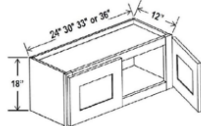
Wall Cabinet Double Doors 18" H
