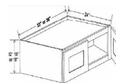
Refrigerator Wall Cabinet Double Doors W331224 W361524 W331524 W361824 W331824 W361224 No shelf
