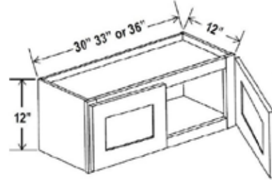
Wall Cabinet Double Doors 12" H
