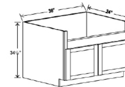
Farmhouse Sink Base
