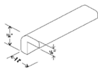
Outside Corner Moulding OCM8
