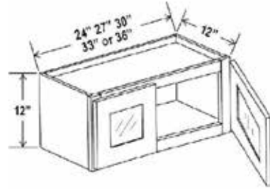
Wall Cabinet Double Glass Doors 12" H
