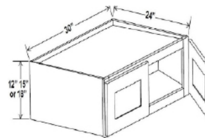
Refrigerator Wall Cabinet Double Doors W301224 W301524 W301824 No shelf
